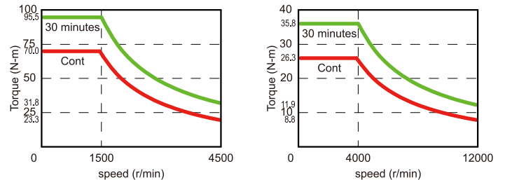
Torque - Speed Characteristic Normal
