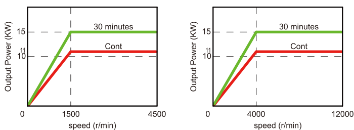
Output Power - Speed Characteristic Normal
